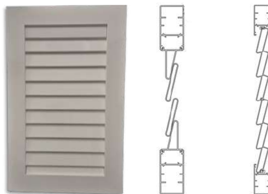
Section lames 54,8/7,1mm Section 59,5/13,8mm
